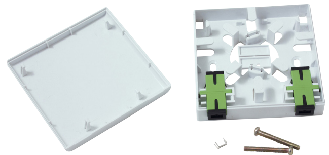
WB-FTTH-2S-SCA
